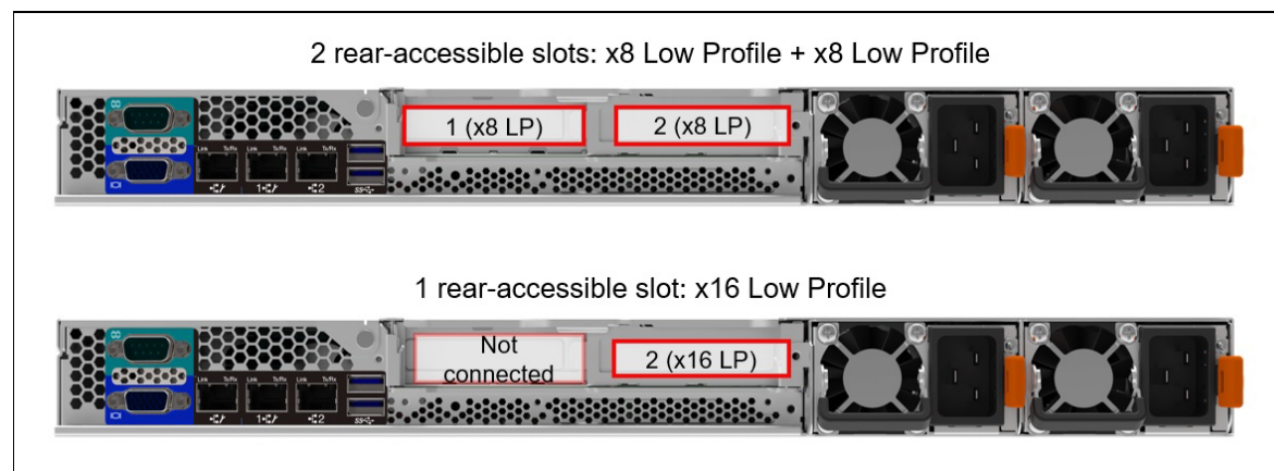
Figure 10. Slot locations
